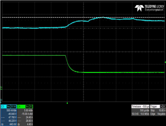
Figure 30: CNS658-MU Transient Response – Vo Deviation V_{IN} = 90Vac, I_O = 100\% \text{ to } 50\% , Output Cap = 330uF/A Ch 3: V_O Ch 4: I_O
