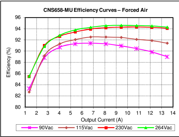
Figure 34: CNS658-MU Efficiency Curves @ 25°C Forced Air V_{IN} = 90 \text{ to } 264Vac , Load: I_O = 0 \text{ to } 13.5A
