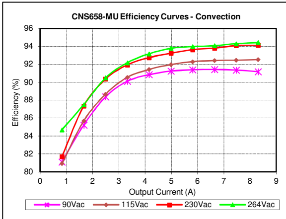
Figure 33: CNS658-MU Efficiency Curves @ 25°C Convection Cooling V_{IN} = 90 \text{ to } 264Vac , Load: I_O = 0 \text{ to } 8.3A
