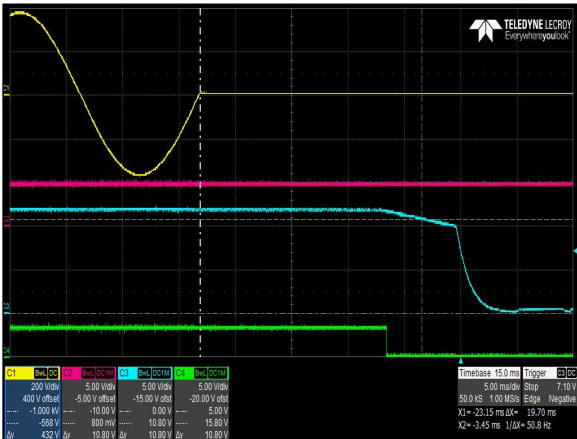
Figure 4: CNS653-ME Hold-up Time – V_{in} = 264Vac / 47Hz / 0^\circ Load: I_O = 54.2A , I_{SB} = 2A Ch 1: V_{IN} Ch 2: V_{SB} Ch 3: V_O Ch 4: PWOK
