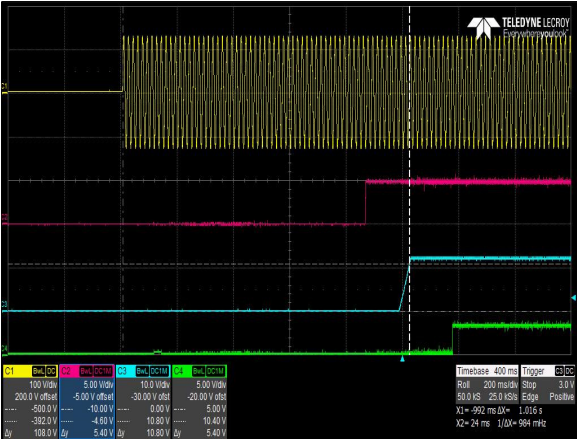
Figure 1: CNS653-ME Turn-on delay by AC Mains – V_{in} = 90Vac Load: I_O = 54.2A , I_{SB} = 2A Ch 1: V_{IN} Ch 2: V_{SB} Ch 3: V_O Ch 4: PWOK
