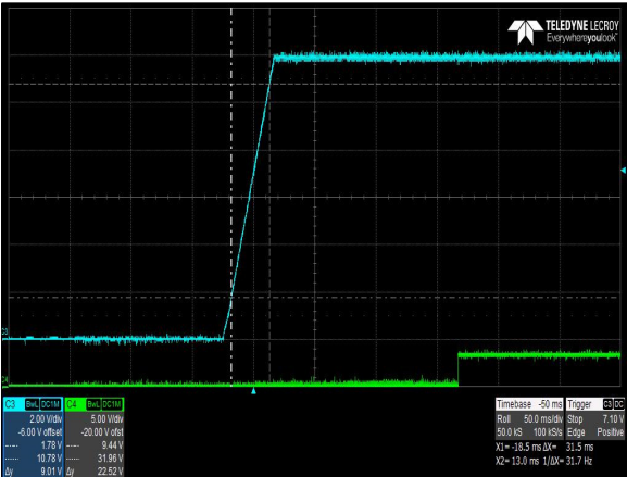
Figure 5: CNS653-ME Output Voltage Startup Characteristic V_{IN} = 90Vac , Load: I_O = 54.2A Ch 3: V_O Ch 4: PWOK
