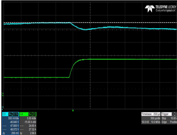
Figure 31: CNS658-MU Transient Response – Vo Deviation V_{IN} = 90Vac, I_O = 100\% \text{ to } 50\% , Output Cap = 330uF/A Ch 3: V_O Ch 4: I_O
