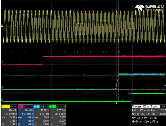
Figure 2: CNS653-ME Turn-on delay by Inhibit – V_{in} = 90Vac Load: I_O = 54.2A , I_{SB} = 2A Ch 1: V_{IN} Ch 2: Inhibit Ch 3: V_O Ch 4: PWOK
