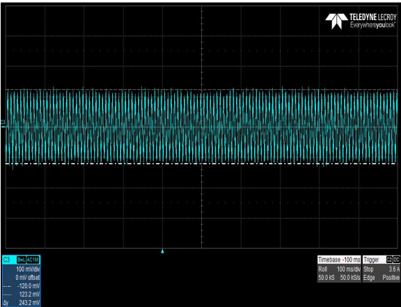
Figure 32: CNS658-MU Ripple and Noise Measurement V_{IN} = 115Vac , Load: I_O = 8.3A Ch 3: V_O
