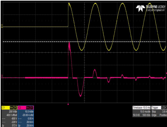
Figure 6: CNS653-ME Inrush Current V_{IN} = 264Vac , Load: I_O = 0A , Turn on angle = 90^\circ Ch 1: V_{IN} Ch 2: I_{IN}
