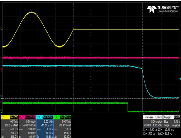
Figure 3: CNS653-ME Hold-up Time – V_{in} = 90Vac / 63Hz / 0^\circ Load: I_O = 54.2A , I_{SB} = 2A Ch 1: V_{IN} Ch 2: V_{SB} Ch 3: V_O Ch 4: PWOK
